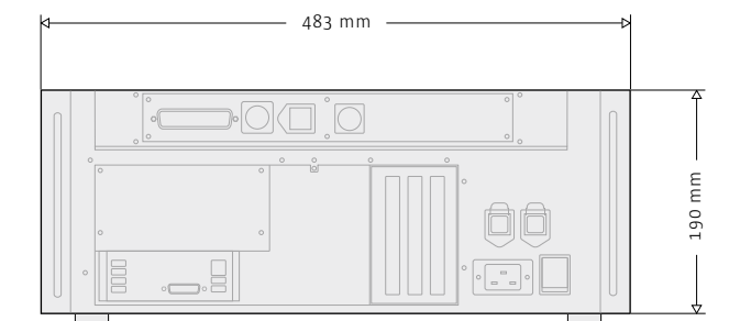
Dimensions of LWR iiwa controller
